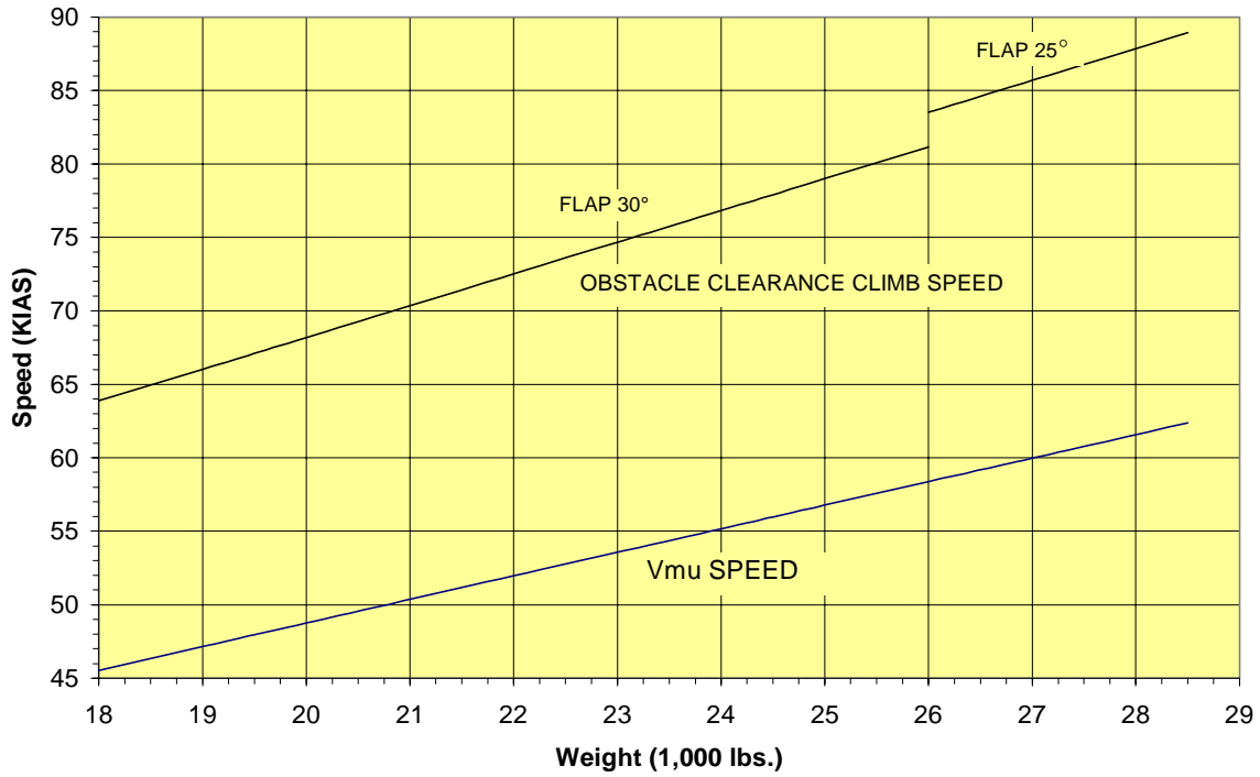
TAKE-OFF SPEED SCHEDULE Figure 8-1
