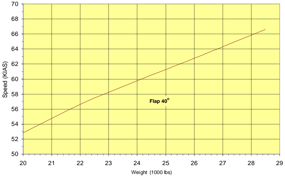
LANDING SPEED SCHEDULE Figure 8-2
