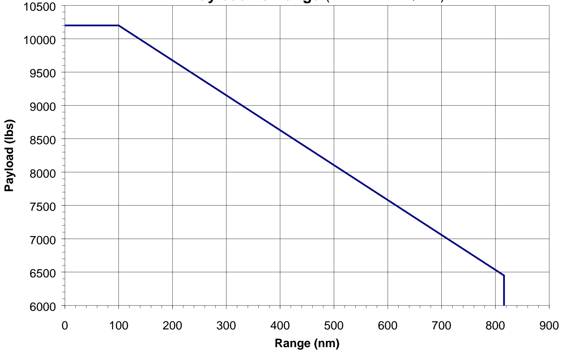
Payload vs Range (at standard cruise power)
